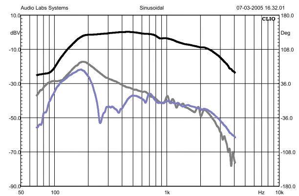
Figure 40: Standard 600-type, driving current response & distortion
