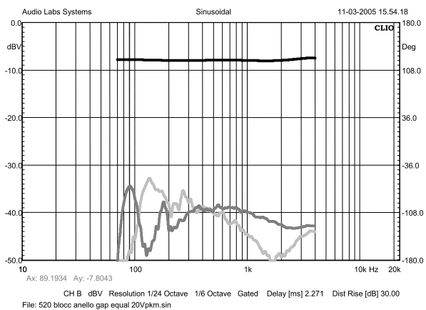
Figure 45: 500-type with shorting ring in the gap, driving current response & distortion
