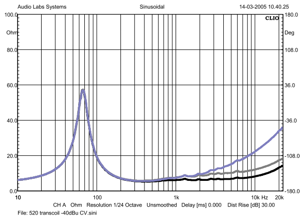
Figure 49: Free air impedance measurement over a 600-type loudspeaker: AIC disconnected (light gray), AIC paralleled to the voice coil (black) or AIC shorted (dark gray).
