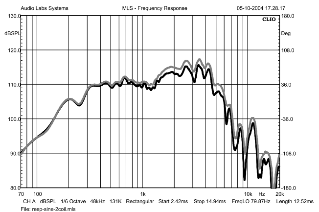
Figure 29: frequency response of a 600 type speaker, without AIC (black) and with AIC (gray)
