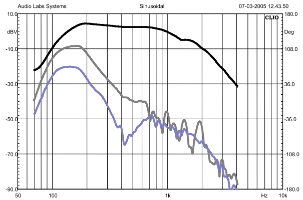
Figure 35: 500-type with AIC, driving current response & distortion
