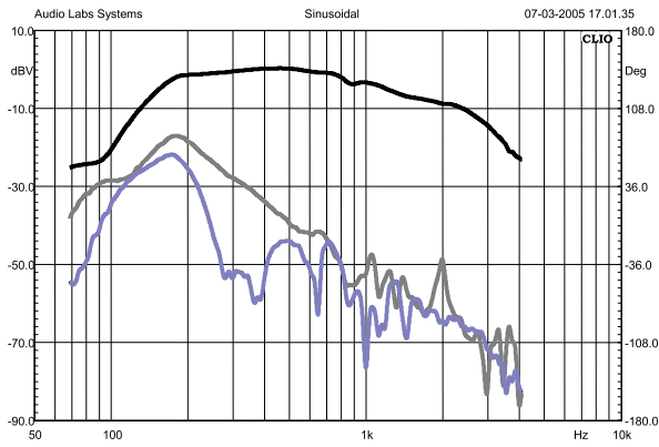
Figure 41: 600-type with AIC , driving current response & distortion
