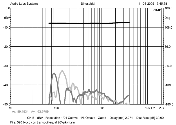
Figure 43: 500-type with AIC , driving current response & distortion
