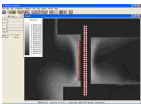
Figure 28: 500-type 2 kHz with AIC, shot 3 - J [A/m 2 ]
