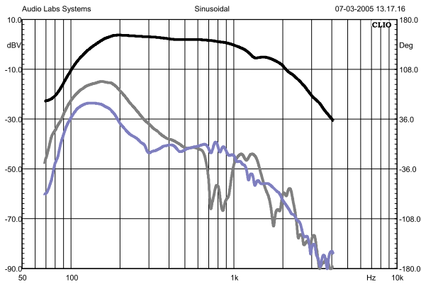
Figure 37: 500-type with ring in the gap, driving current response & distortion
