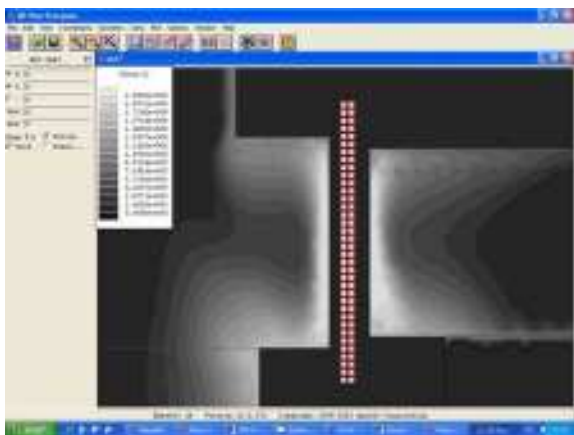
Figure 25: 500-type normal 2 kHz - shot 3 - J [A/m 2 ]
