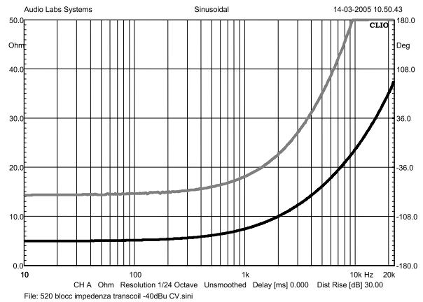
Figure 51: Impedance curves of the blocked speakers: the impedance of the voice coil (black) and the impedance of the AIC coil (gray curve)
