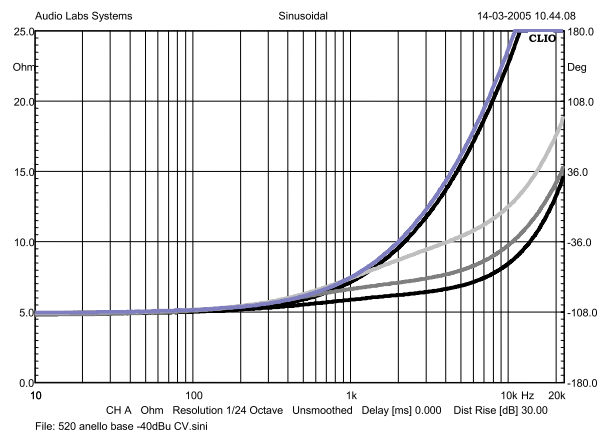
Figure 50: Impedance curves of the blocked speakers
