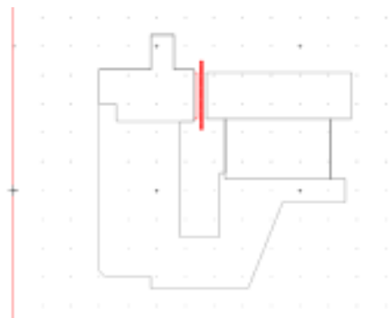
Figure 3: Model of a 500 type magnetic circuit with a shorting ring in the gap instead of the A.I.C. coil
