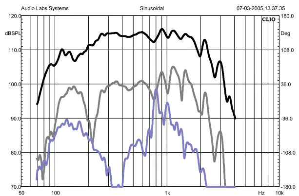
Figure 32: 500-type with ring under the pole piece
