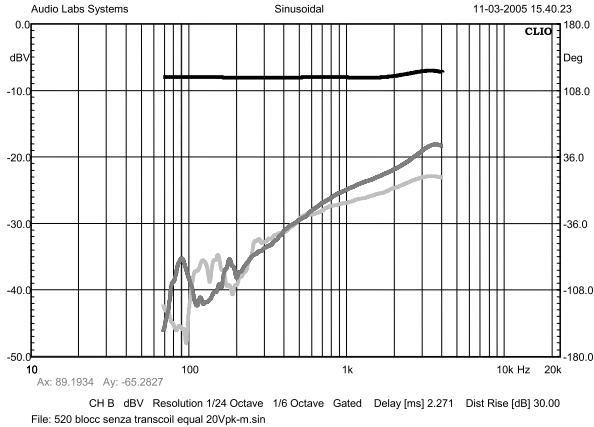
Figure 42: Standard 500-type, driving current response & distortion
