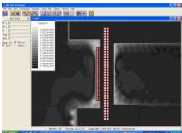
Figure 27: 500-type 2 kHz with AIC, shot 2 - J [A/m 2 ]
