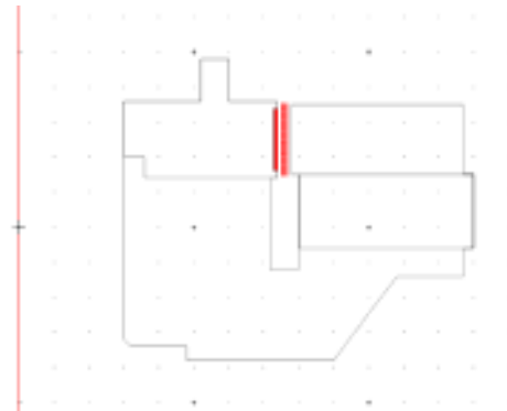
Figure 1: Model of a 600 type magnetic circuit.
