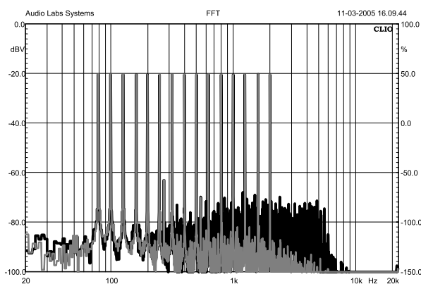
Figure 46: driving current FFT multi-tone test over a 500-type with AIC (gray) and without it (black).
