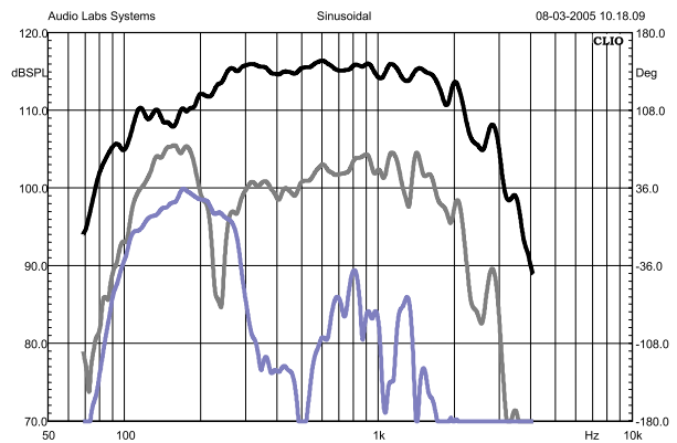
Figure 31: 500-type with AIC, response and distortion
