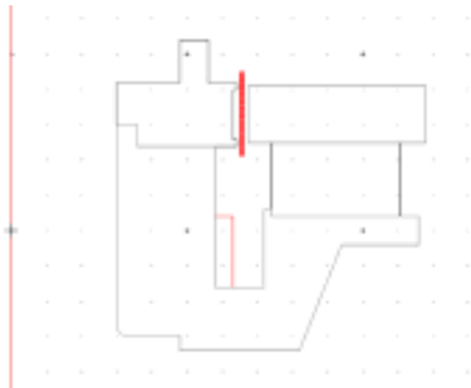
Figure 4: Model of a 500 type magnetic circuit with a shorting ring at the base of the pole piece instead of the A.I.C. coil
