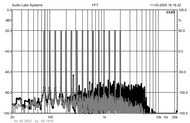
Figure 47: driving current FFT multi-tone test over a 500-type with a ring in the gap (gray) and without it (black).
