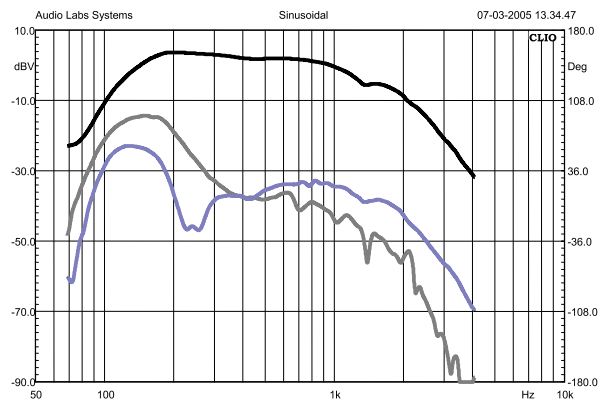
Figure 36: 500-type with ring under the pole piece, driving current response & distortion
