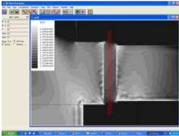
Figure 5: 500-type normal 250Hz - shot 1 – B [T]
