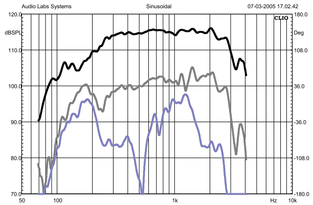
Figure 39: 600-type with AIC, response and distortion
