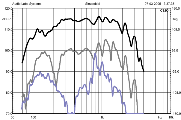
Figure 33: 500-type with ring in the gap
