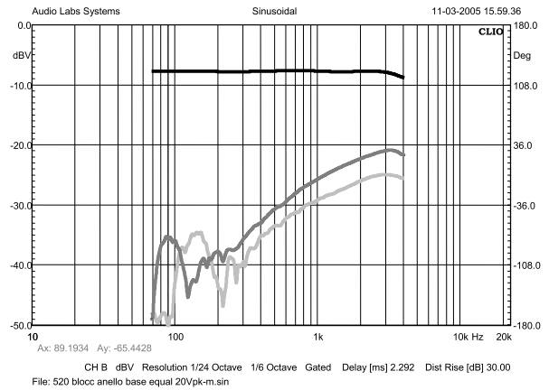
Figure 44: 500-type with ring under the pole piece , driving current response & distortion
