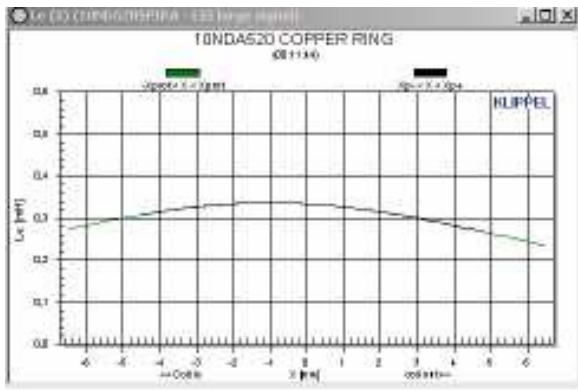
Figure 53: L_e vs. displacement in a 500-type speaker with the ring under the pole piece
